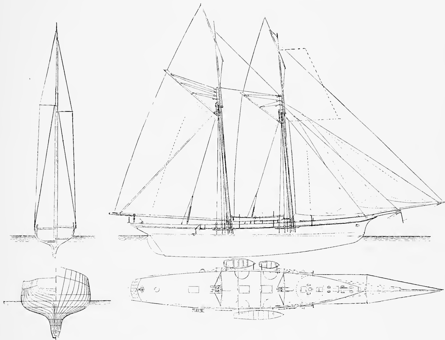
THE CELEBRATED FRENCH SCHOONER YACHT VELOX.
